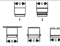
BEARING CAP TYPES
